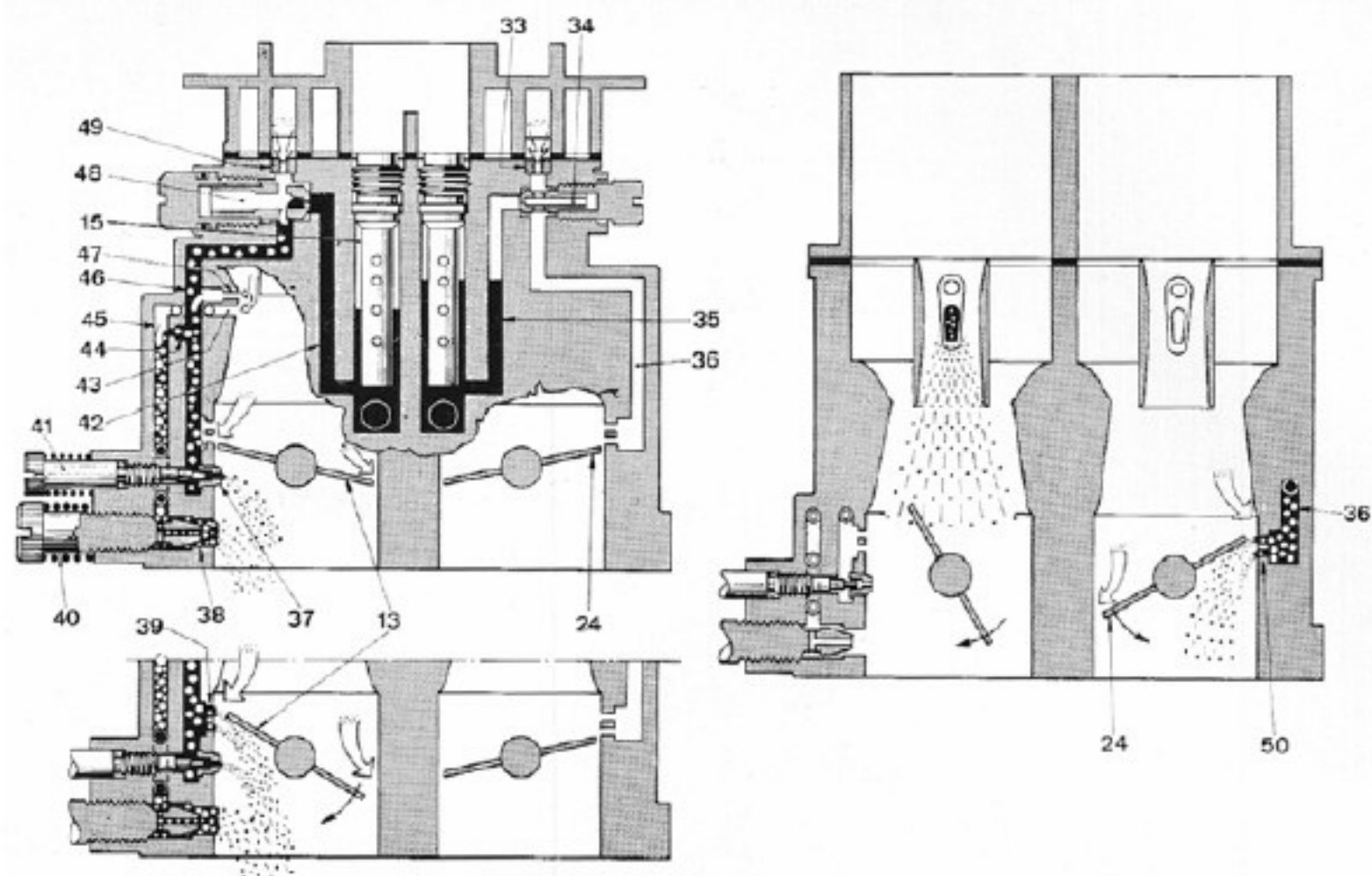
Figure 22: DMS Progression
