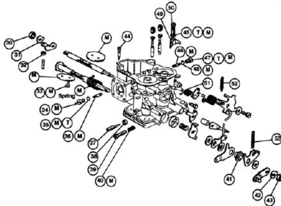
Figure 13: DHS A Jetting, Throttle Mechanisms, and Internal Parts
