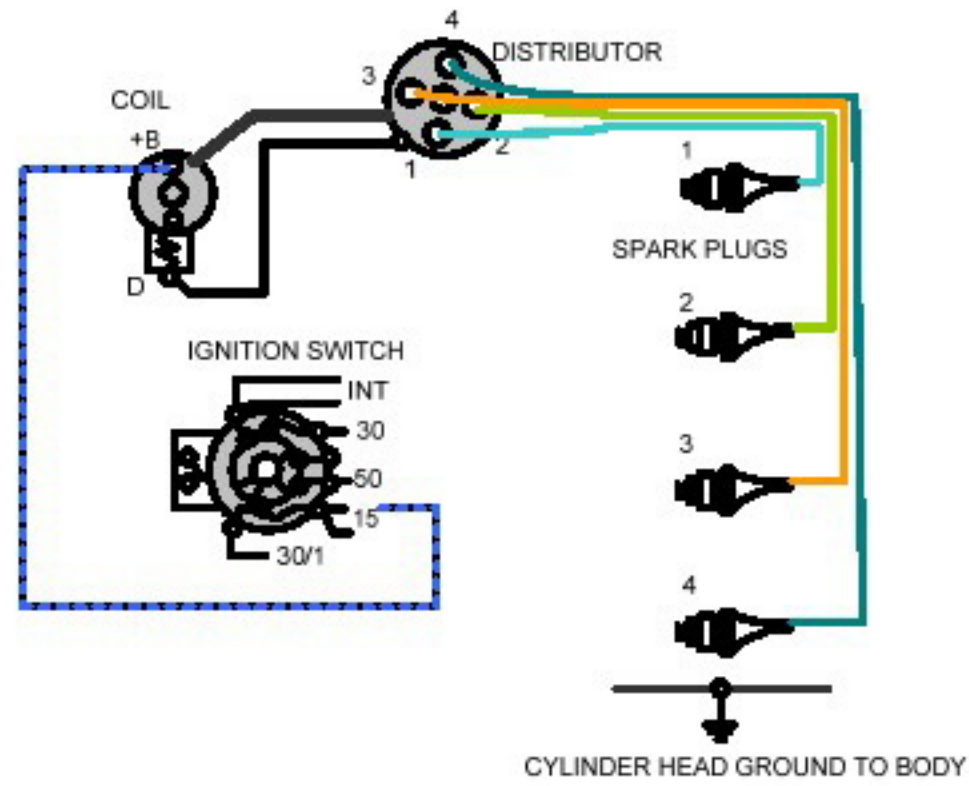
Figure 44: Ignition Electrical Diagram for the 1967-1973 Spider
