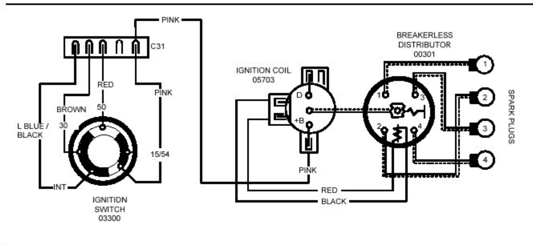
Figure 46: Ignition Electrical Diagram for the 1979-1985 Spider
