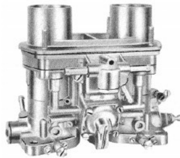
Figure 14: IDF Carburetor Side View
