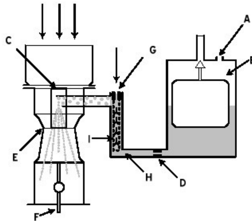
Figure 3: Air Bleed Correction. A Float Chamber Vent, B Fuel Bowl or Chamber, with Float, C Spray Tube, D Fuel Jet, E Venturi, F Throttle, G Air bleed jet, H Well for emulsion tube, I Emulsion Tube
