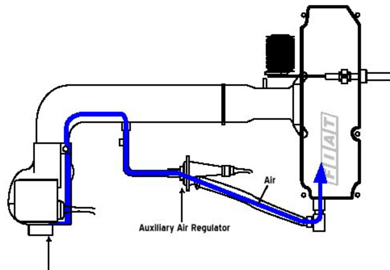
Figure 35: Warm-up Operation in the Bosch L-Jetronic System
