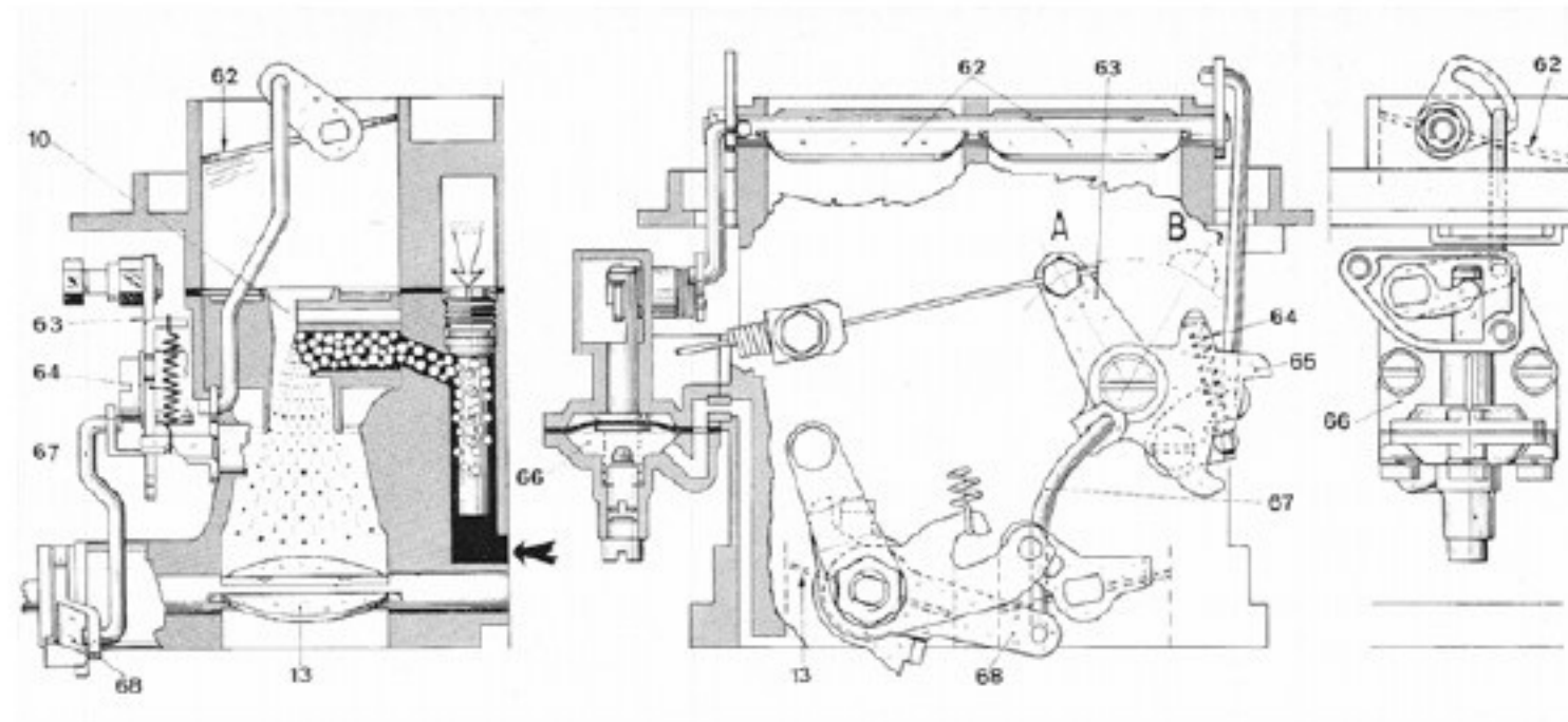
Figure 24: DMS Starting
