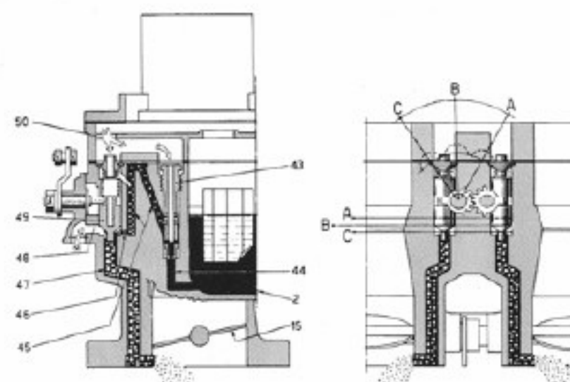
Figure 18: IDF Cold Start Devices
