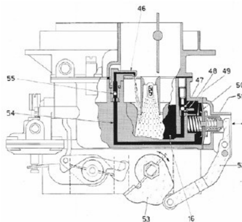
Figure 29: ADF Acceleration
