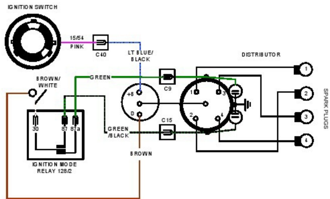
Figure 45: Ignition Electrical Diagram for the 1974-1978 Spider
