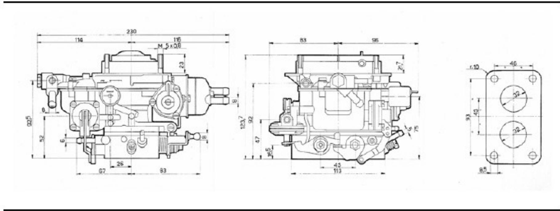
Figure 32: ADF Dimensions
