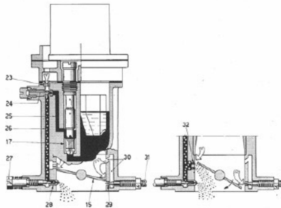
Figure 16: IDF Progression
