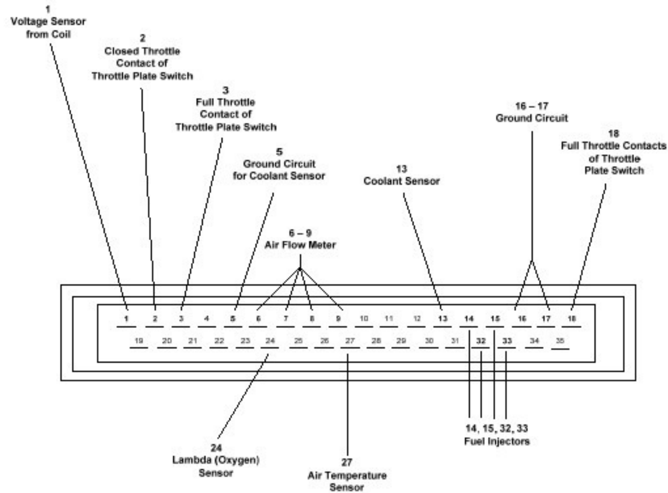
Figure 38: Primary Connections on the Electronic Control Unit
