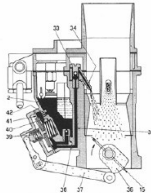
Figure 17: IDF Acceleration
