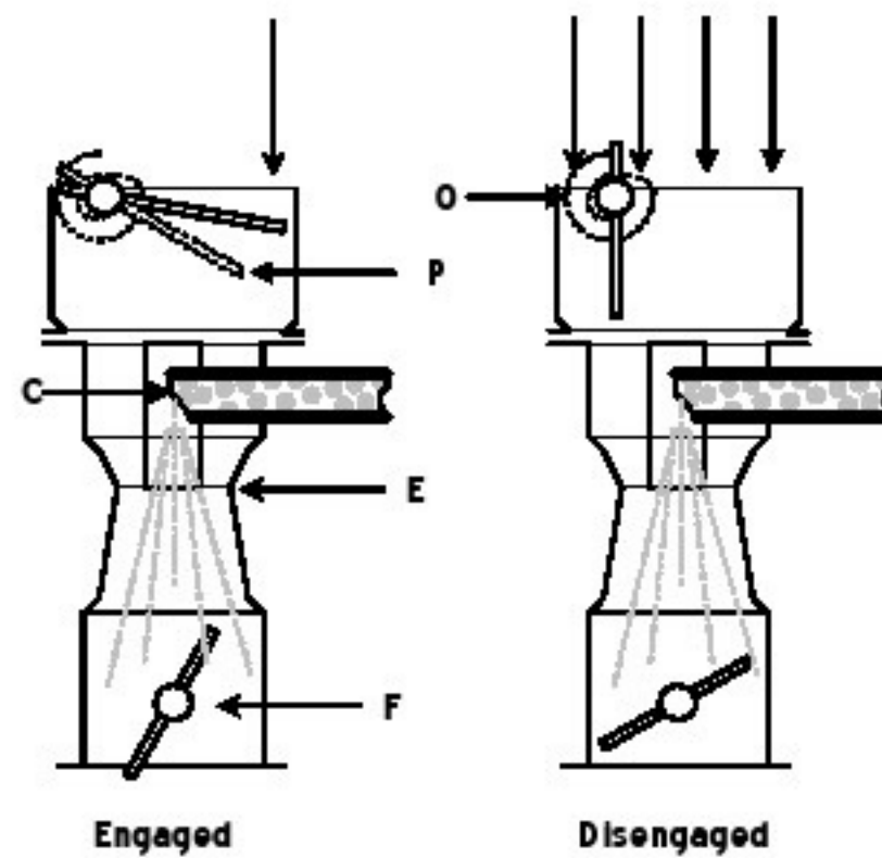
Figure 7: Offset choke, P choke valve, C spray nozzle, E venturi, F throttle, O calibrated spring
