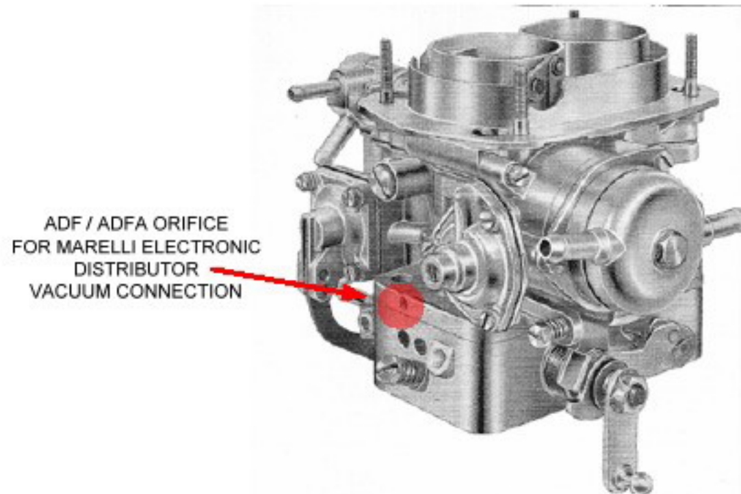
Figure 47: Location of port for vacuum advance
