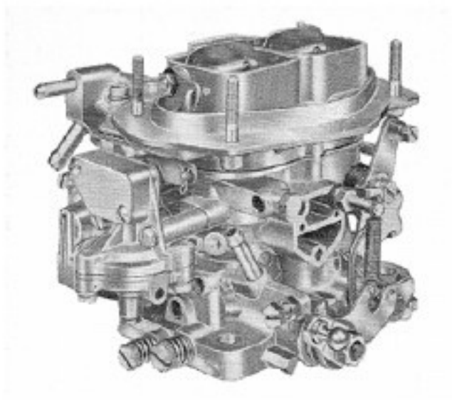
Figure 20: DMS Carburetor Side View
