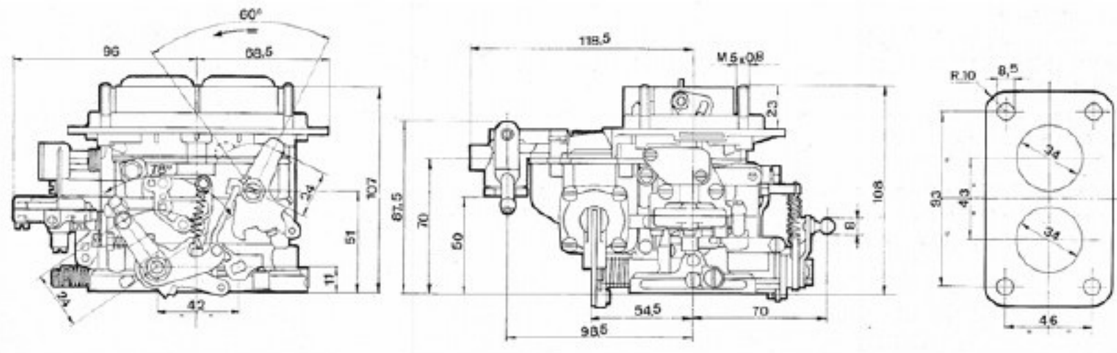
Figure 25: DMS Dimensions
