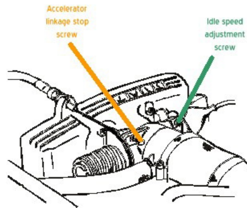
Figure 37: Idle speed controls on the Spider 2000
