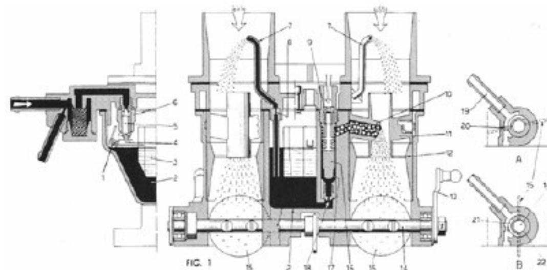
Figure 15: IDF Normal Operation
