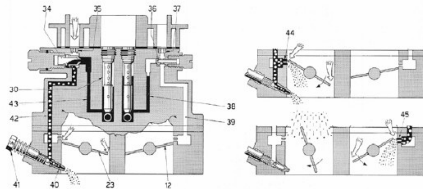
Figure 28: ADF Idle Speed and Progression
