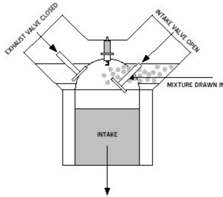
Figure 41.1: Intake
