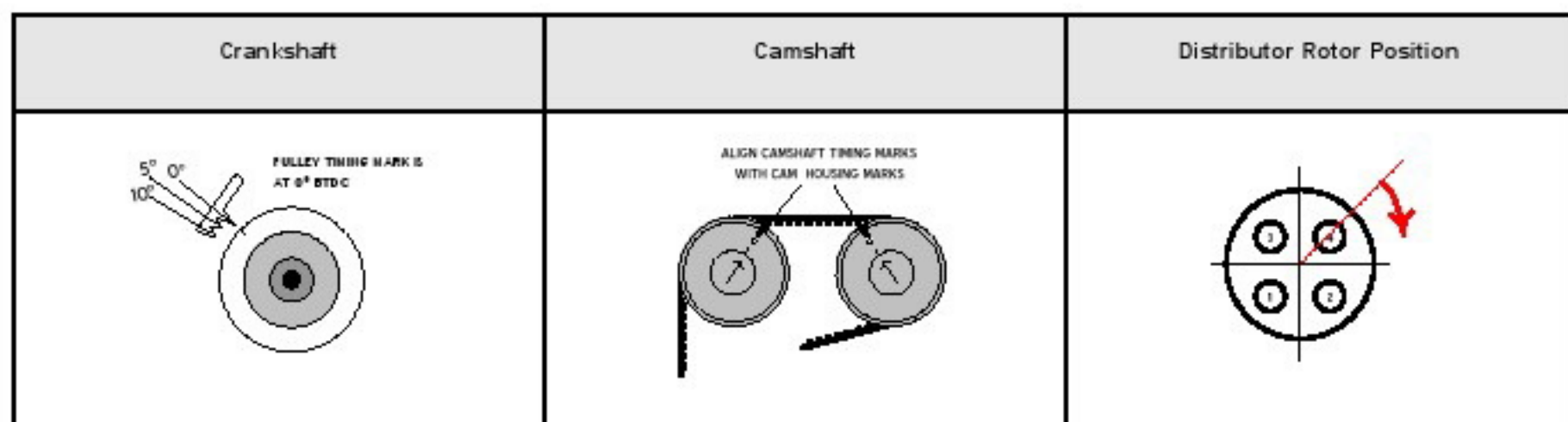
Figure 42: Initial Ignition Setting
