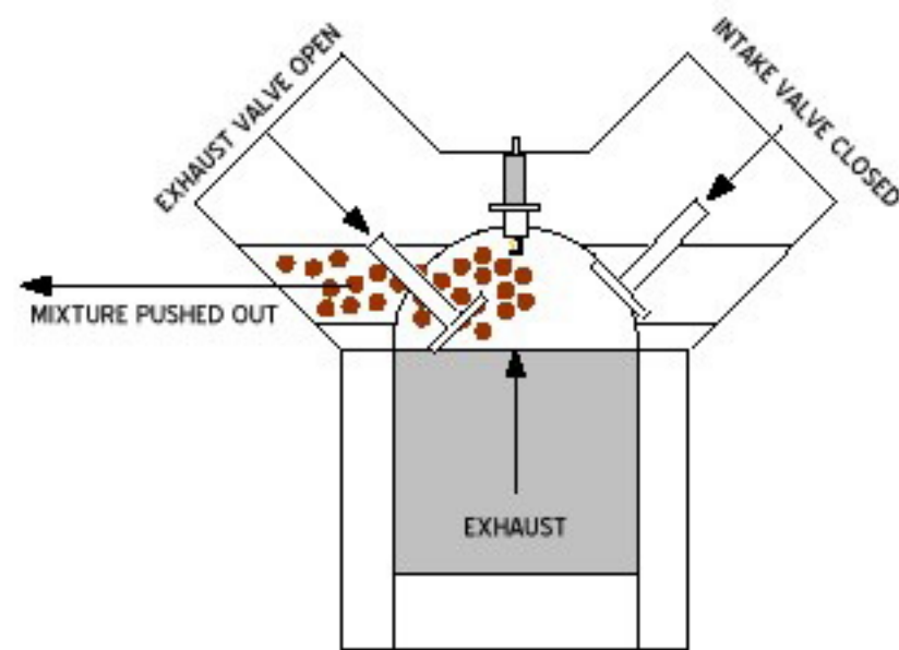
Figure 41.4: Exhaust
