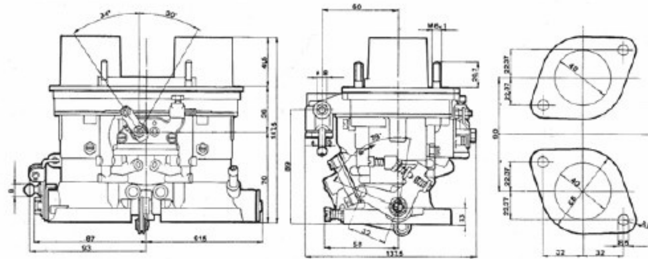
Figure 19: IDF Dimensions
