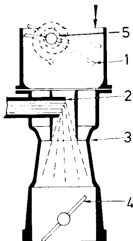
Fig. 1.10 The Weber strangler type choke (Sec 4)
