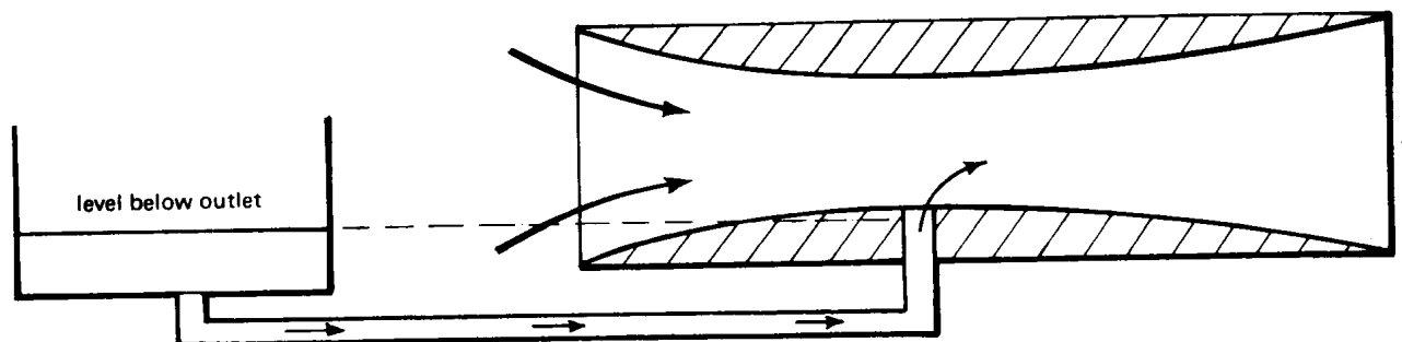
Fig. 1.3 The principle of fuel flow into a venturi (Sec 3). Large arrows indicate air flow, small arrows indicate fuel flow
